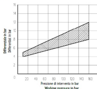
PRESSIONE DIFFERENZIALE • DIFFERENTIAL PRESSURE FT-IPNB-630
