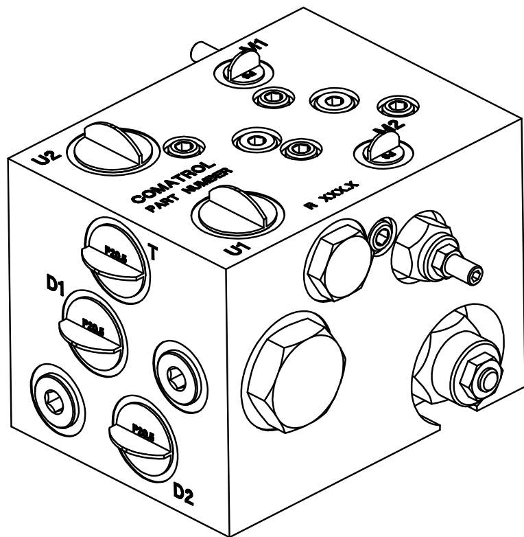
Isometric View
