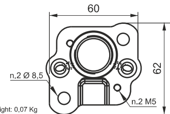
Aluminium adapter flange for group 0 Code: E60513025
