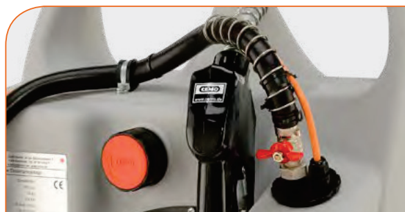
anti-kink protection + swivel joint + shut-off valve
