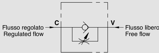
SCHEMA IDRAULICO HYDRAULIC DIAGRAM
