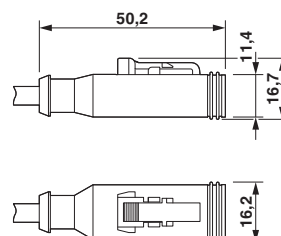
DEUTSCH DT06-2S, top view and side view
