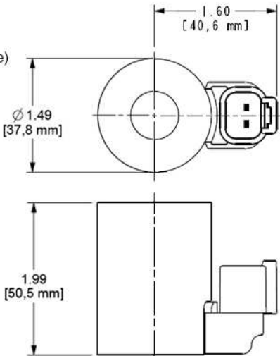
DC COIL (without TVS Diode)
