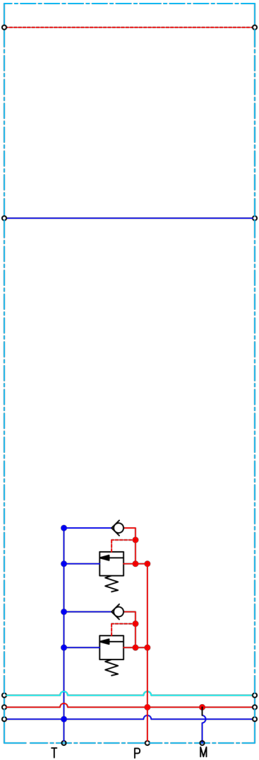
Technical specification for PVPM 48
