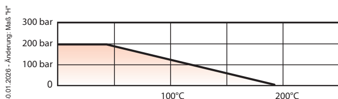
Druck- Temperatur- Diagramm / Pressure- Temperature Chart
