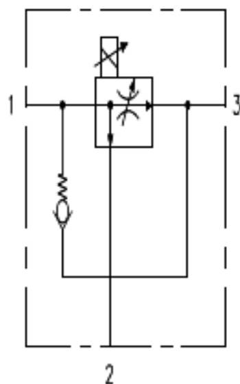
HG755 CAV TVTP50
