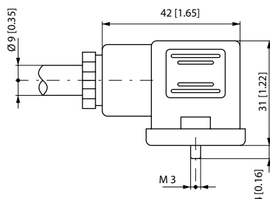
TYPE C CONNECTOR
