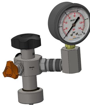
Analogic pressure gauge connected through quick adapter (example)
