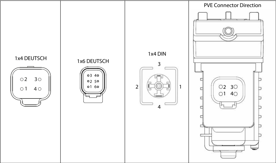
Connector diagrams
