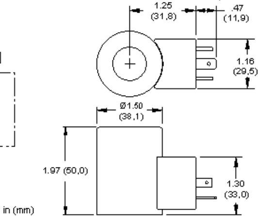
DC COIL
