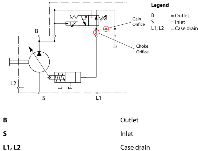
Fan Drive Control Schematic
