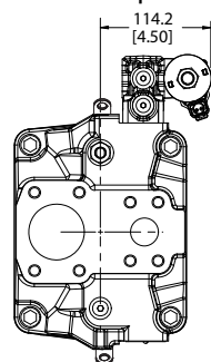
Axial Endcap Counterclockwise
