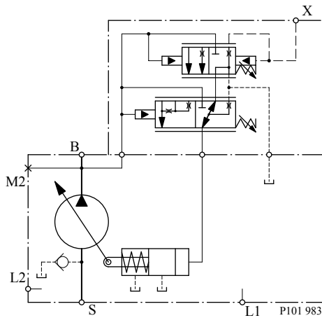
LB Schematic
