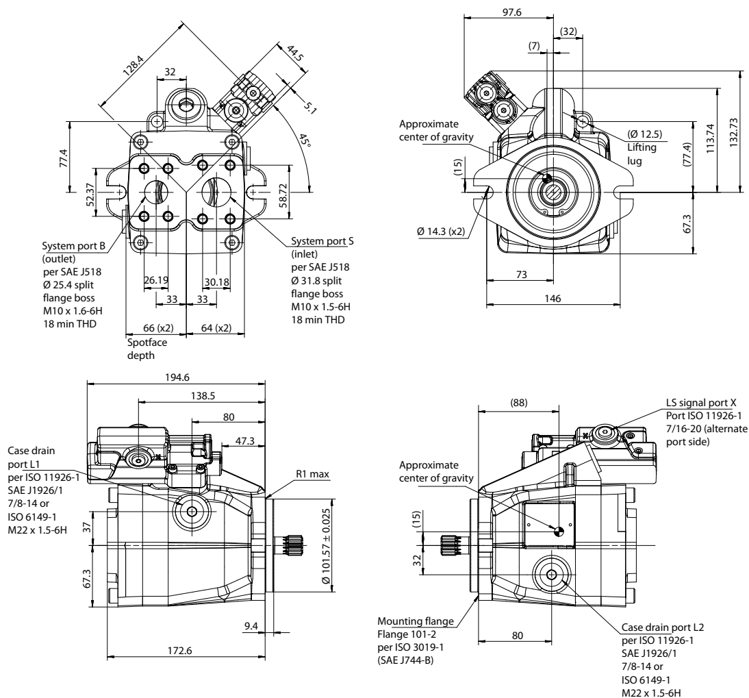
K2 split flange axial endcap and LS control
