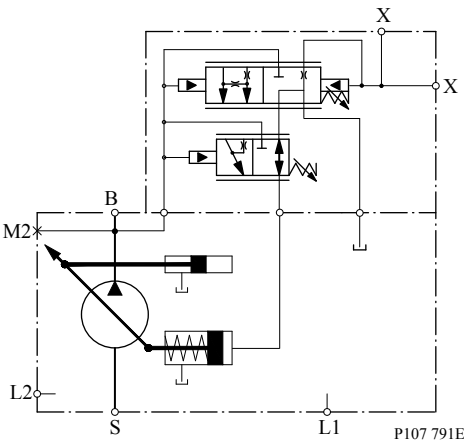
Schematic
