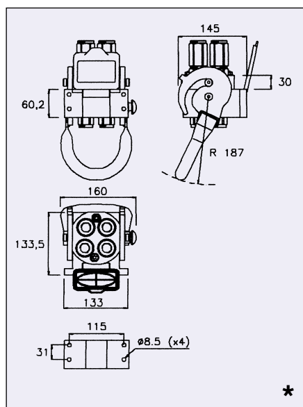
Version 3P508 Four lines 1/2" size
