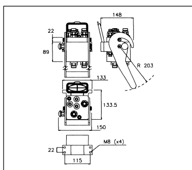
Version 2P5S3 Three lines 1/4" size Two lines 3/8" size 3/8" - 3/8" shunt
