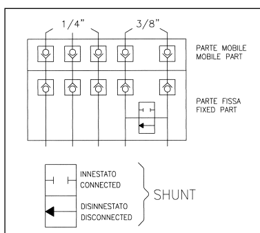
Hydraulic layout
