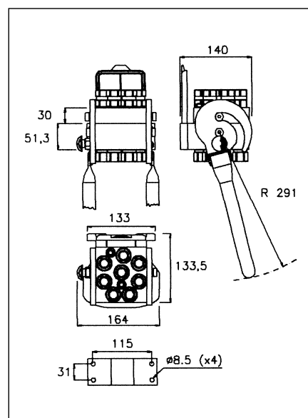
Version 2P5068 Eight lines 3/8" size
