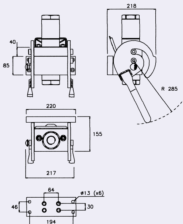
Version 3P124 One line 1 1/2" size
