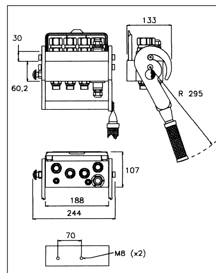
Version 2PS08 Five lines 1/2" size
