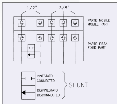
Hydraulic layout
