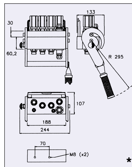
Version 3PS08 Five lines 1/2" size
