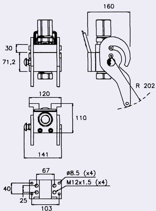
Version 3P116 One line 1" size
