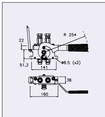
Version 3PB06 Two lines 3/8" size
