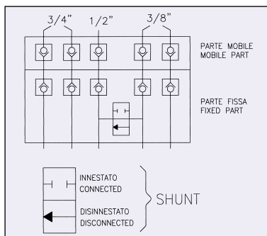
Hydraulic layout
