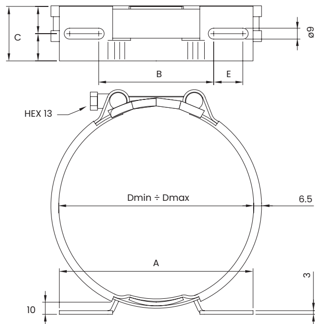
Technical Drawing / Fastening collar light series
