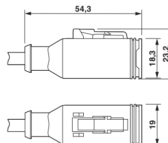
Dimensional drawing
