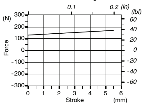
Force-stroke diagram
