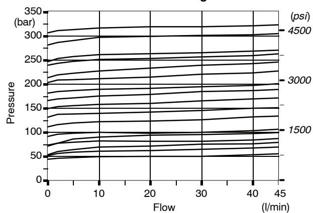
Pressure-flow diagram
