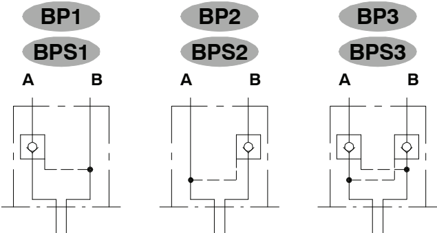
BP3 configuration Example of pressure on port A and port B to tank
