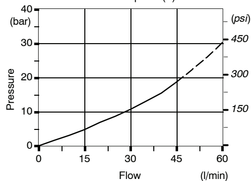
Pressure drop
