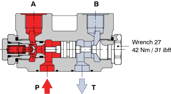
BP1 configuration Example of pressure on port A and port B to tank
