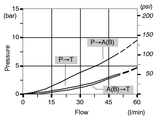
Pressure drop curve
