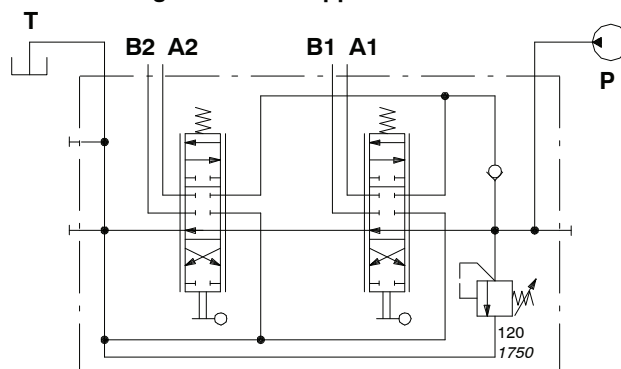
Configuration with upper inlet and outlet
