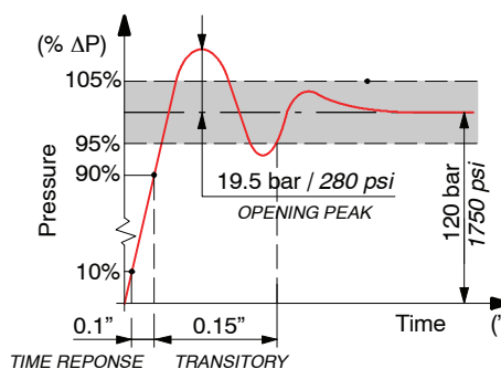
Time response
