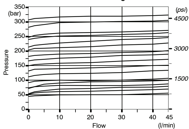
Pressure-flow diagram
