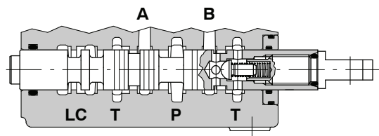
A-B→T (floating detent)
