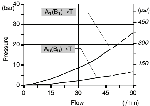
Pressure drop A(B)→T on 6 sections directional valve
