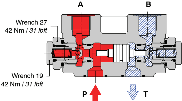
BP3 configuration Example of pressure on port A and port B to tank
