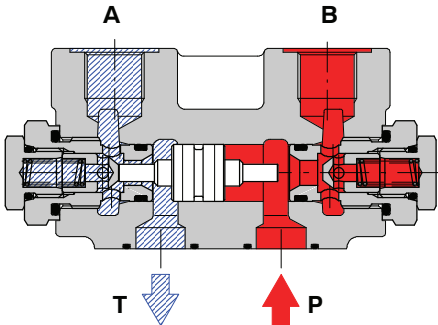
Example of pressure on port B and port A to tank
