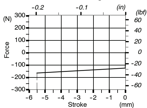
Force-stroke diagram
