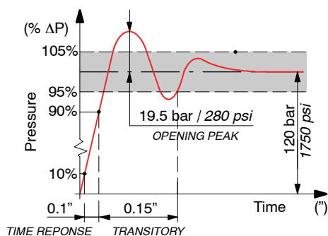
Time response
