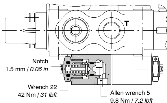
Spring nr. 2 (green band)
