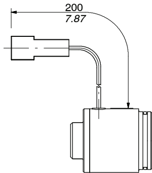
Coil with AMP Fastin-Faston connection
