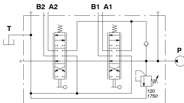
Description example: SD5/2-P(KG3-120)/ED-18L/ED-18L/AEK
