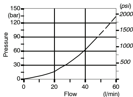
Pressure drops
