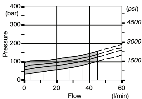
Pressure drops
