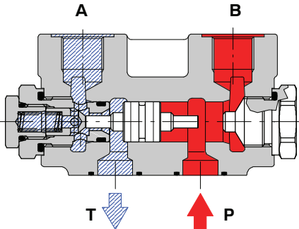
Example of pressure on port B and port A to tank
