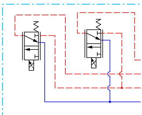
PVHC schematic
