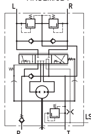
Closed Center - Non Reaction HKULS.../5DT
