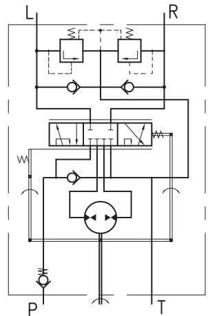
"Close Center - Non Load Reaction" HKUS.../7 ser.3
