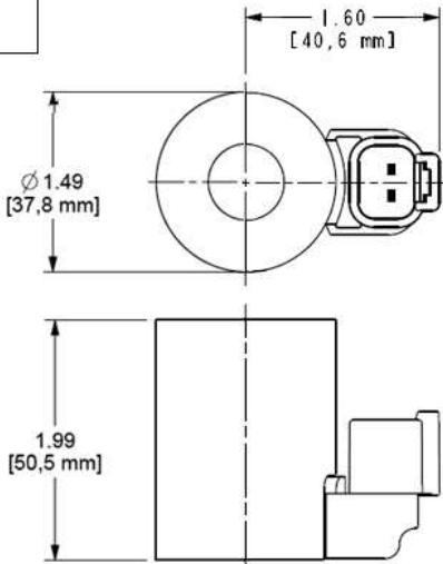
DC COIL
