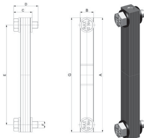
Reference Drawing B
