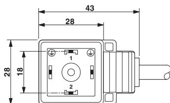
Valve connector, type A, side view
